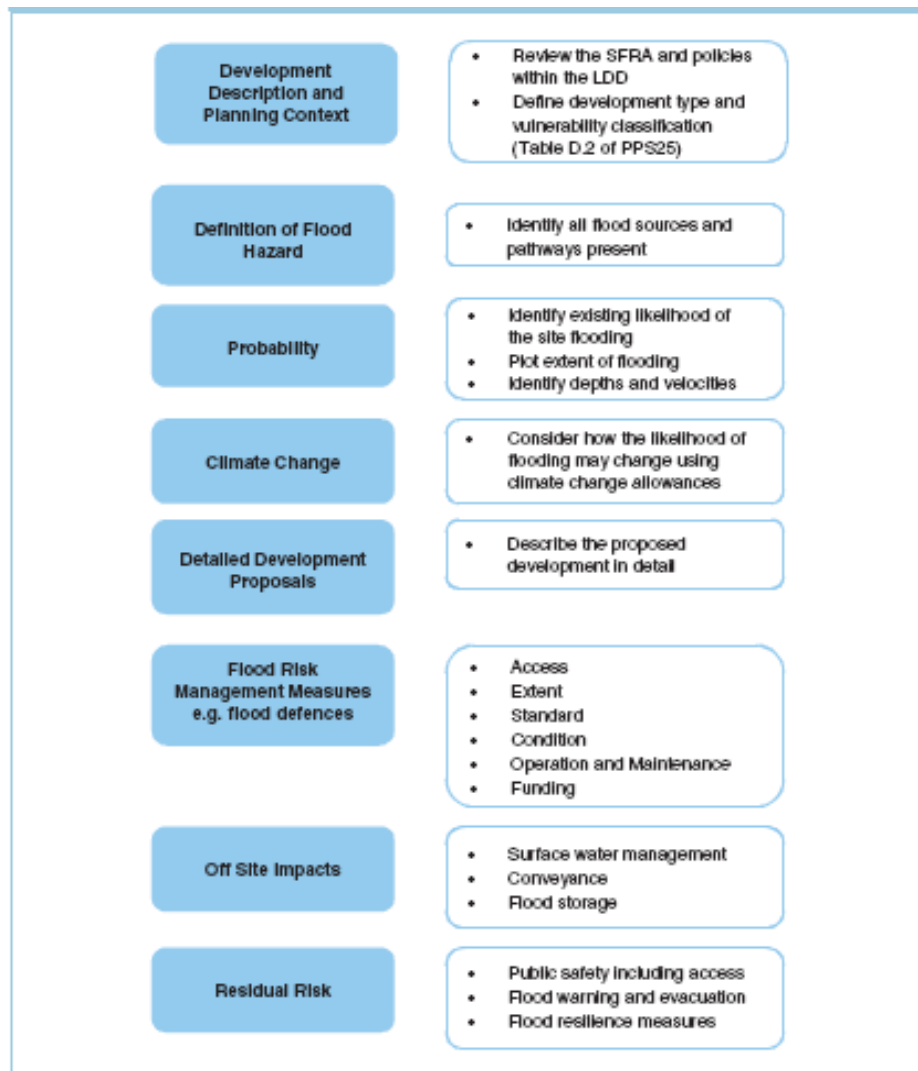
Figure C.1: Scope of Site-Specific Flood Risk Assessment
