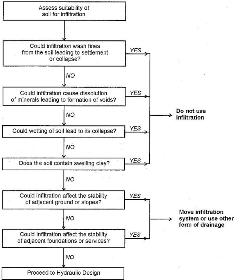
Figure C.2: Decision guide for the use of infiltration systems
